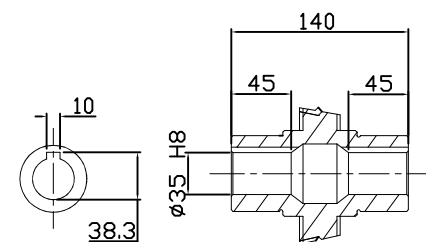
OUTPUT HOLLOW SHAFT
