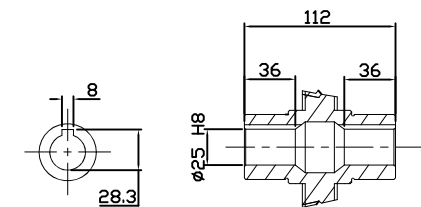
OUTPUT HOLLOW SHAFT
