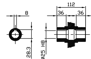
OUTPUT HOLLOW SHAFT
