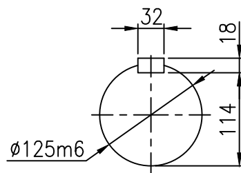
OUTPUT SHAFT
