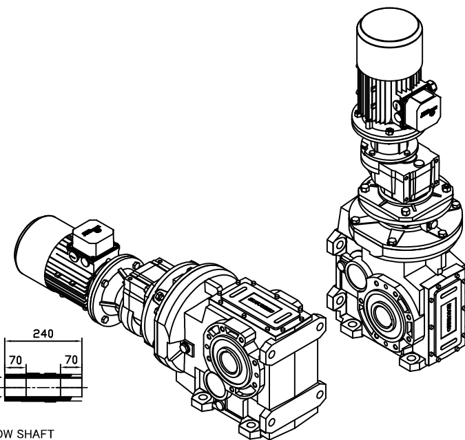
OUTPUT HOLLOW SHAFT
