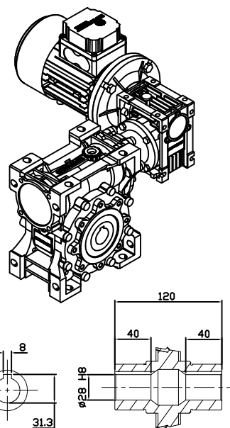
OUTPUT HOLLOW SHAFT
