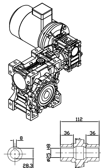
OUTPUT HOLLOW SHAFT
