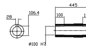
OUTPUT HOLLOW SHAFT
