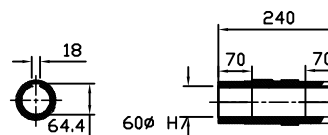
OUTPUT HOLLOW SHAFT
