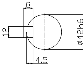
OUTPUT SHAFT
