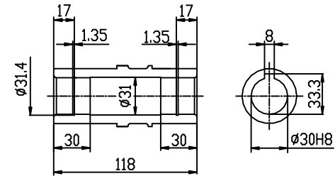
OUTPUT SHAFT
