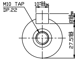
OUTPUT SHAFT
