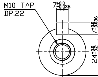
OUTPUT SHAFT
