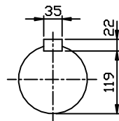
OUTPUT SHAFT
