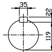
OUTPUT SHAFT
