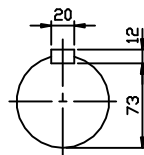
OUTPUT SHAFT
