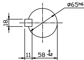
OUTPUT SHAFT
