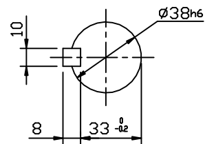
OUTPUT SHAFT
