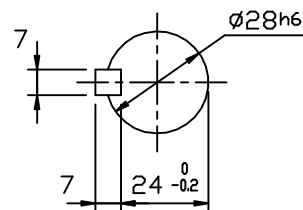
OUTPUT SHAFT
