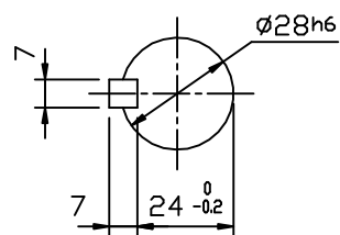
OUTPUT SHAFT
