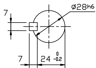
OUTPUT SHAFT
